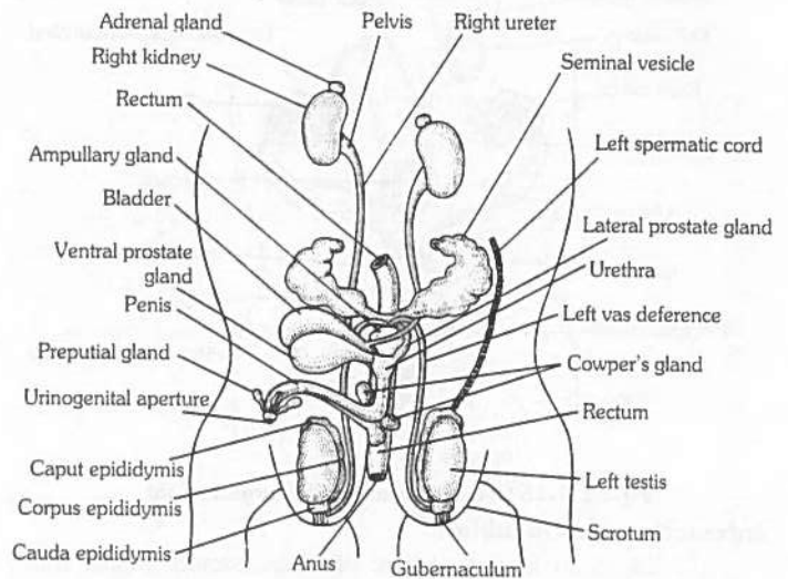
Fig : 2.4-14 Male urinogenital organs of rat
