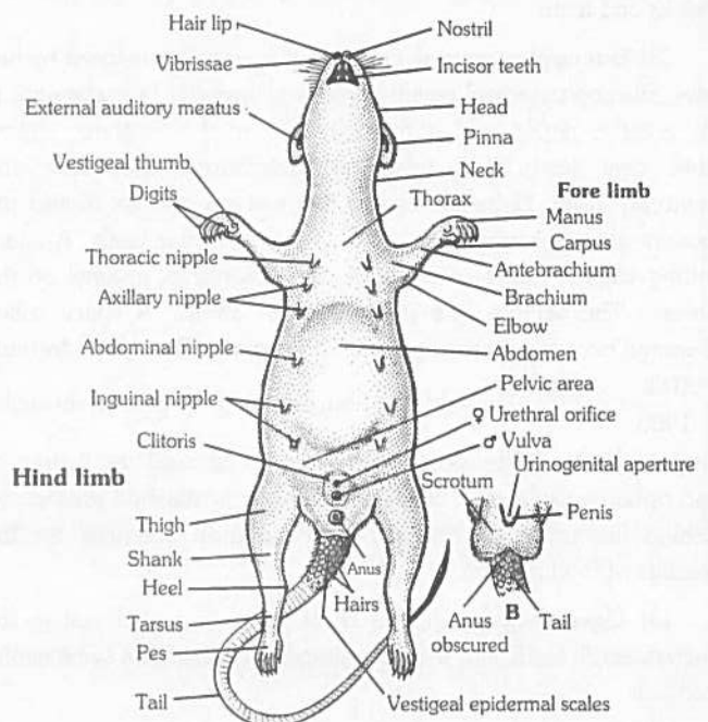
Fig : 2.4-8 External morphology of rat (a) Ventral view of female rat; (b) Ventral view of pelvic region of male rat
