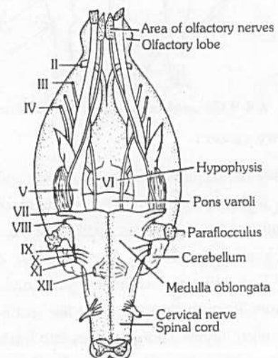
Fig : 2.4-13 Ventral view of the brain of Rat
